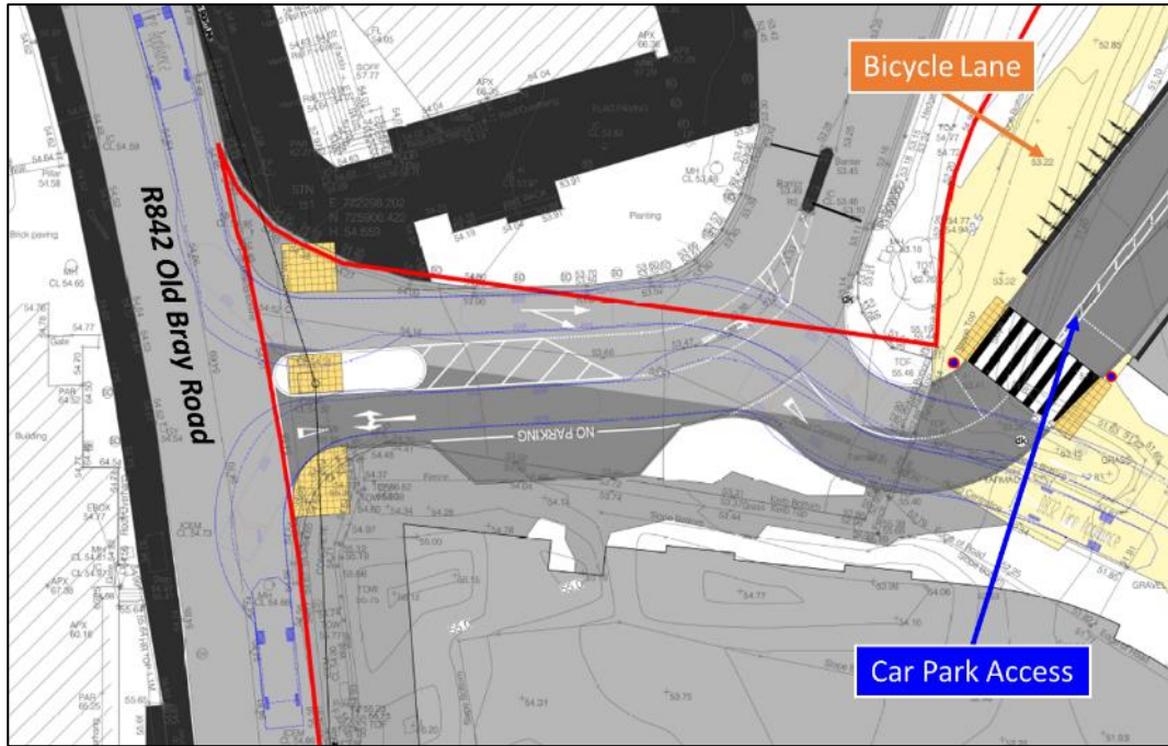
Figure 4.1: Site Access Junction Layout
